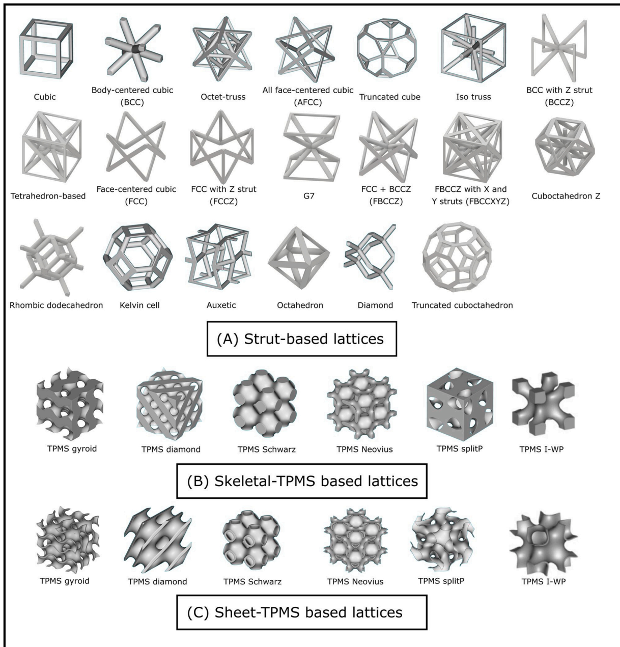
Fig. 6. Various architectures of lattice structures (A) Strut-based lattice cells are shown in the first three rows. (B) Skeletal- and (C) sheet-tripty periodic minimal surfaces (TPMS).
